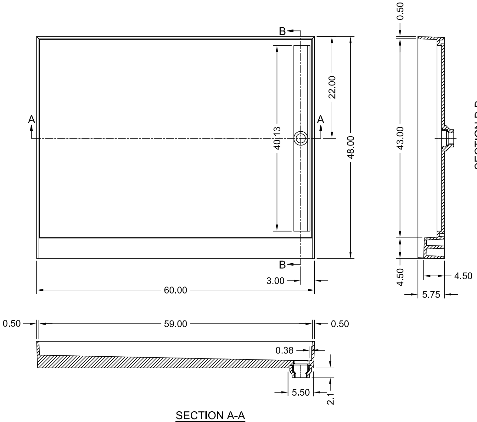
SECTION B-B
